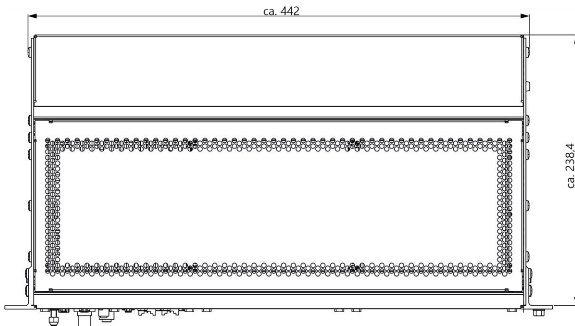
Fig. 4/3: Top view
