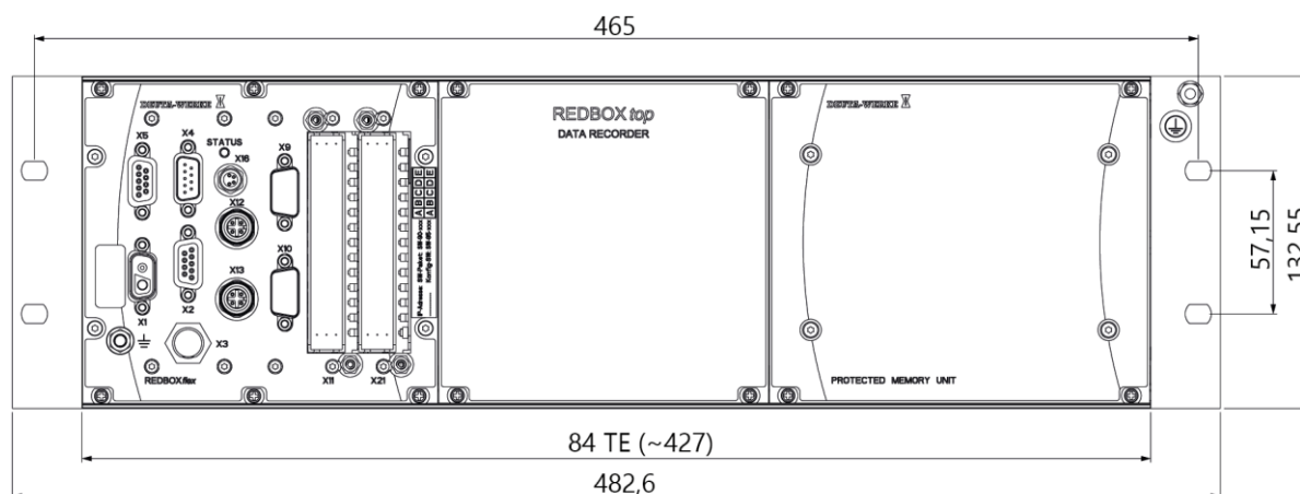
Fig. 4/1: Front view
